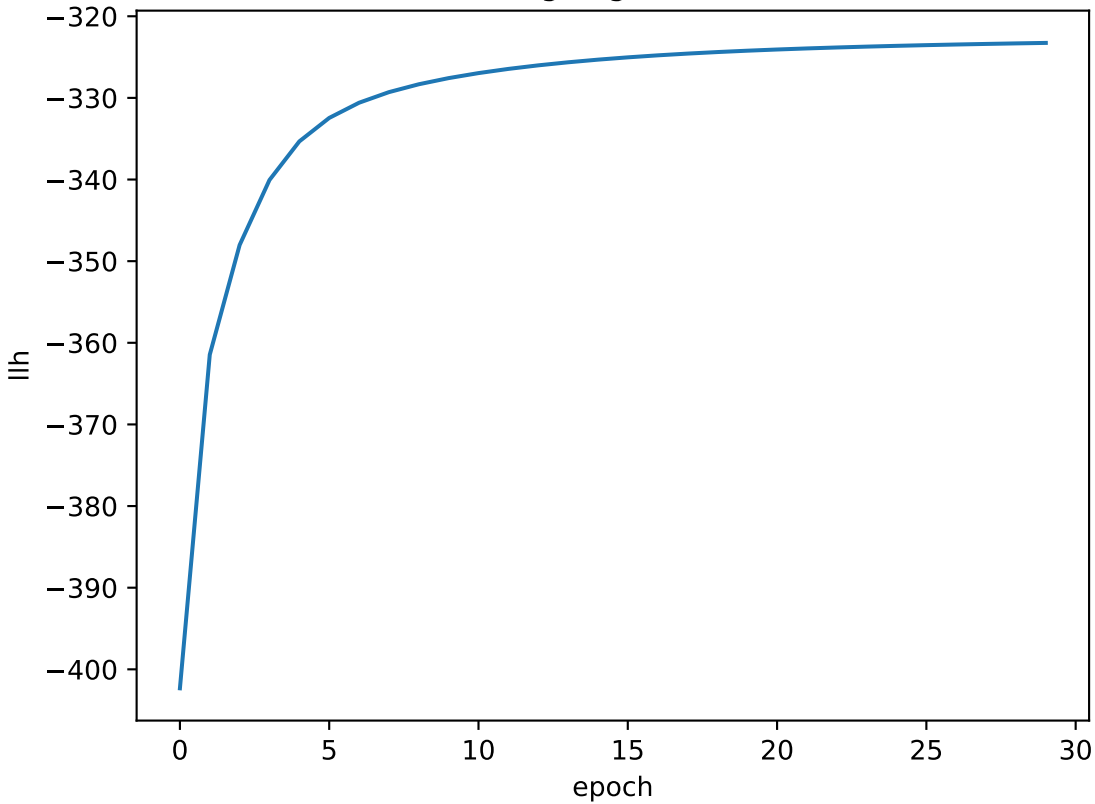
Training Log-likelihood
